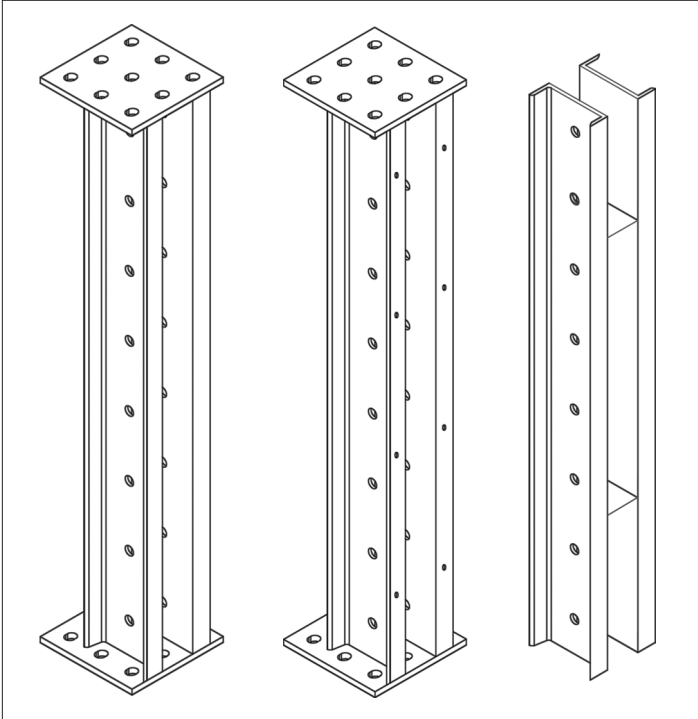
Walers (left to right) - Butt Plate Waler, Pafco-style Waler and Double Channel Waler.
