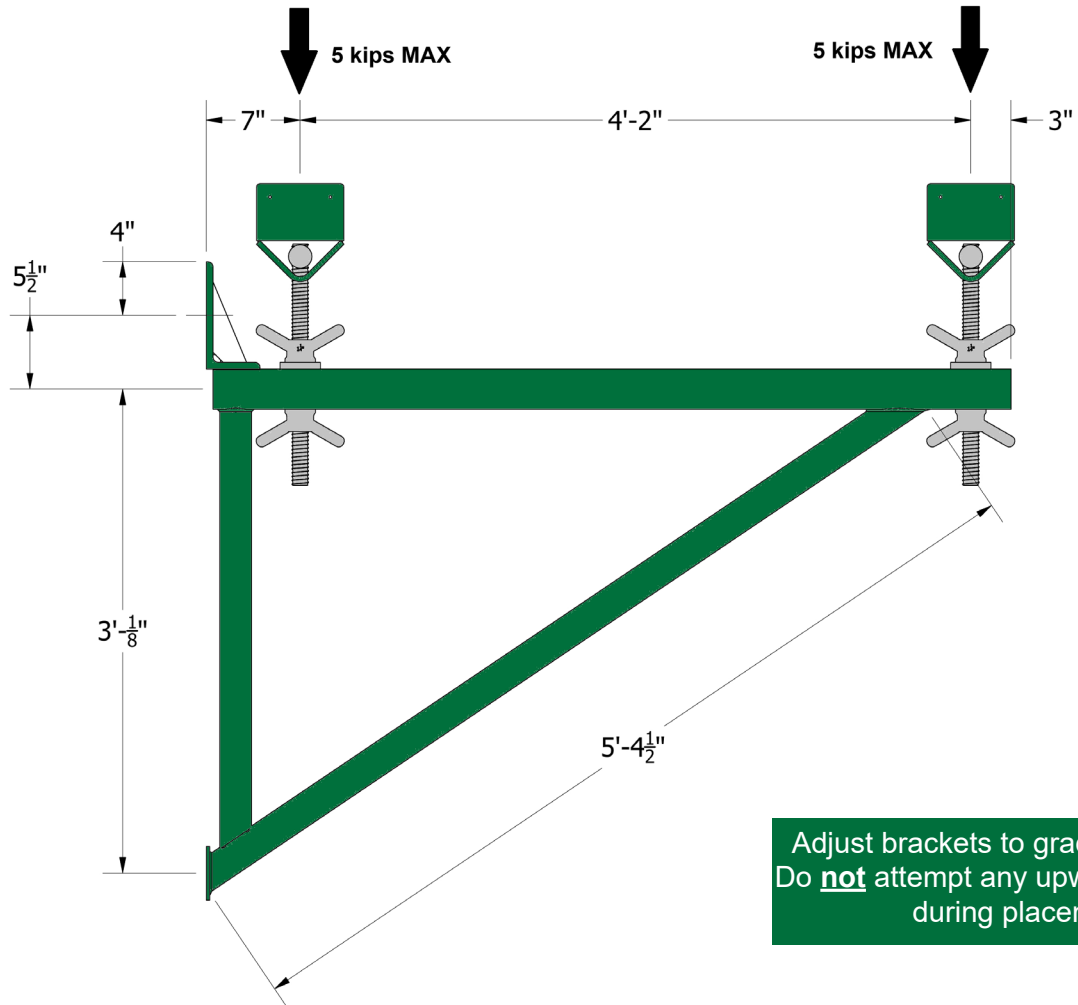
SureSaddle 10 kip Bridge Overhang Bracket - 5 kips max load per saddle jack
