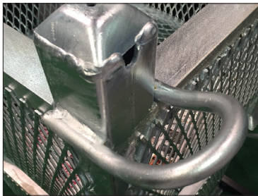
Corner lugs provide reliable attachment points for lifting and moving the basket.
