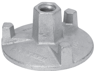
Euro Wing Nut Plate
